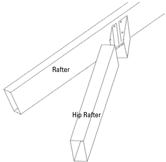
Top hip to Dutch gable end rafter
