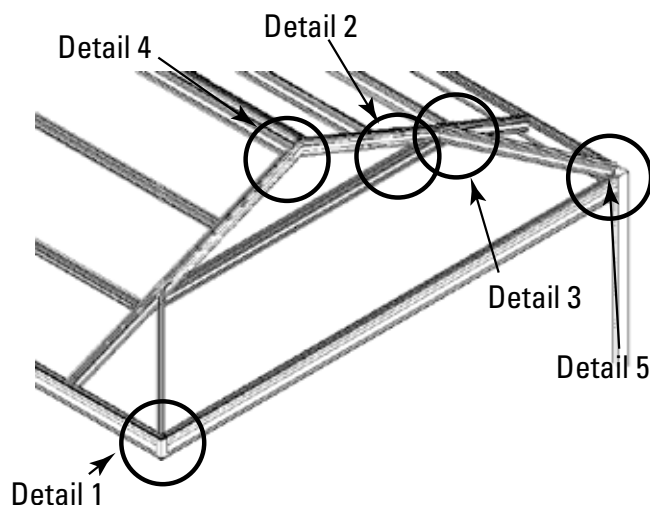
Beams in Dutch End
