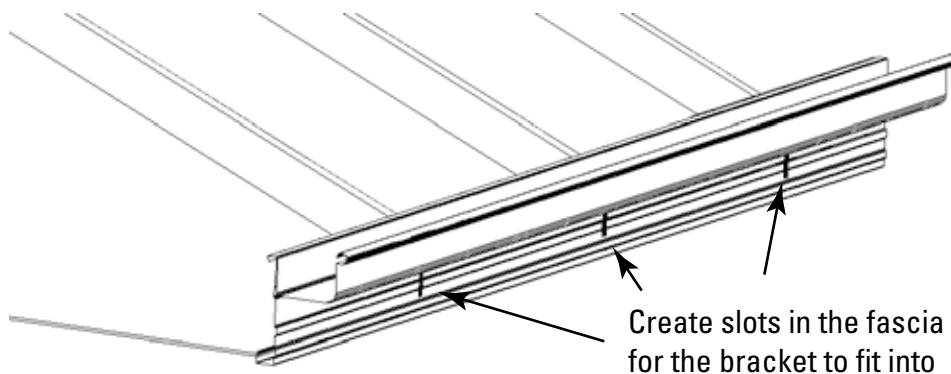
Existing fascia with new slots
