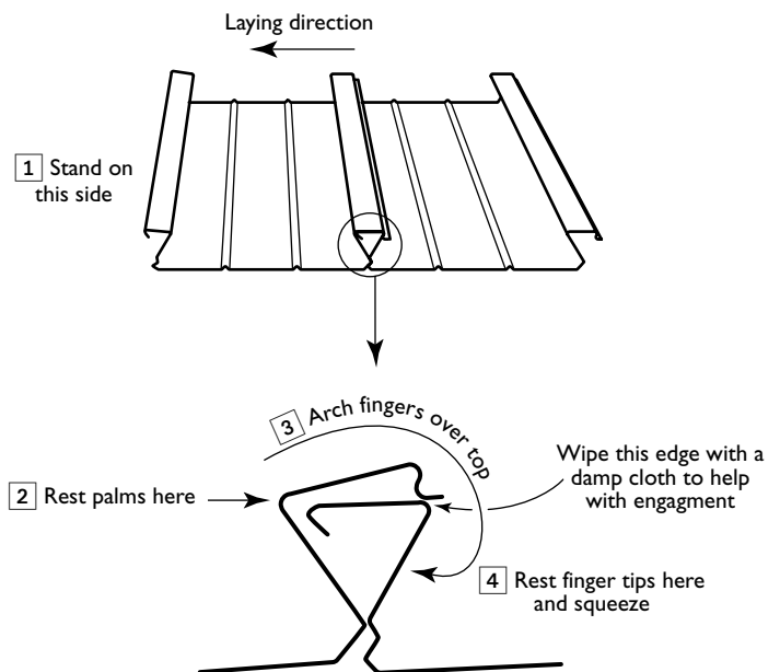
Interlocking ribs
