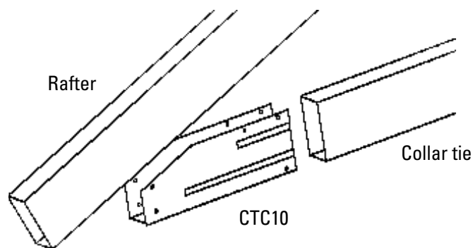
Detail 2 Collar tie
