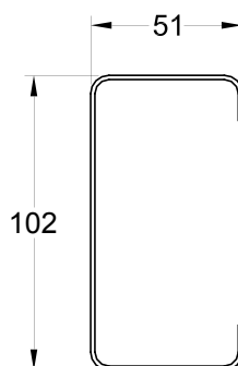
Rafter strengthener (CHS102)
