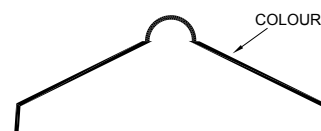
Ridge Capping for Custom Orb (CRIDGE)
