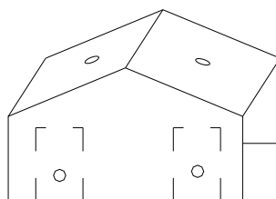
Gable Post Top Connector CON100G
