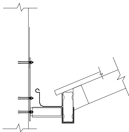
Rail support to wall-up
