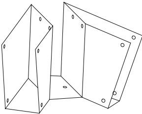
Purlin/Hip Rafter Connector (HRU10)
