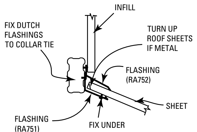
Elevation at Dutch hip end
