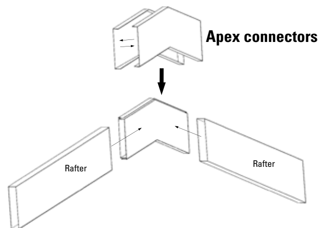
Apex connection
