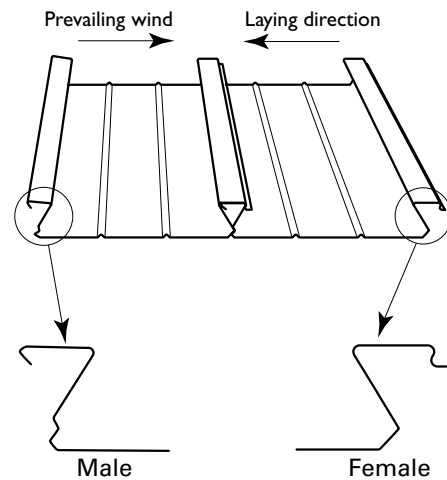
FLATDEK ribs
