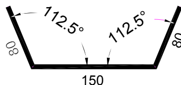
Internal Apex Flashing (DLFLA)
