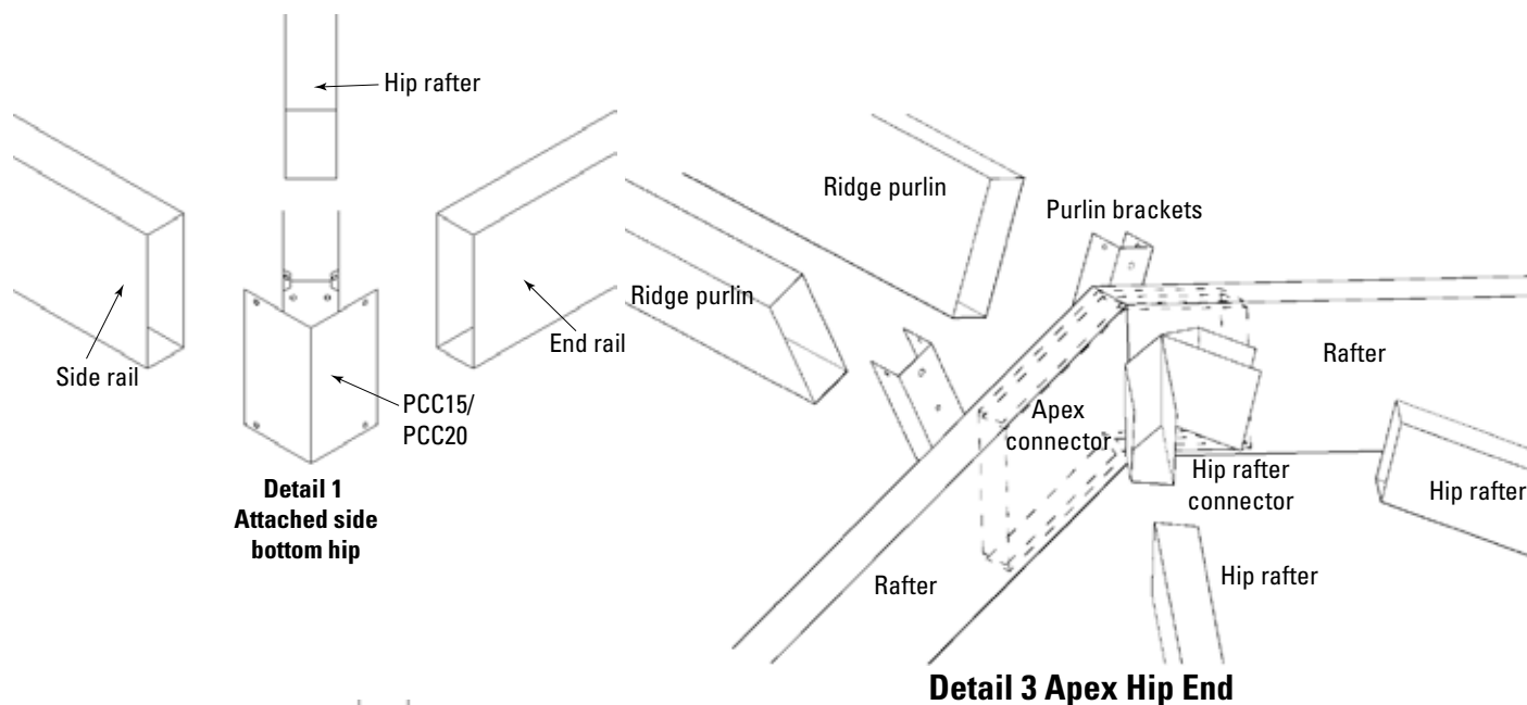
Hip End
