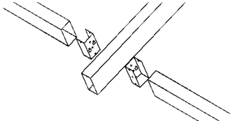
Intermediate purlins to rafter
