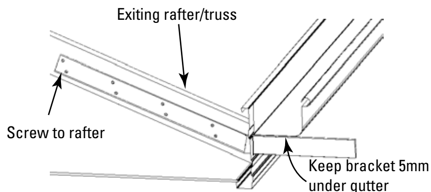
After bracket has been inserted through fascia
