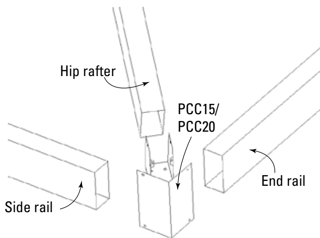
Detail 1 Attached side - bottom hip
